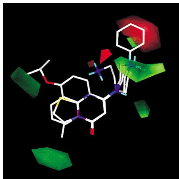
Figure 1. STDEVxCOEFF isocontour steric plots for models P 3 (for the colour code see text). Contour levels as follows: red 0.035; green 0.025; compounds 5d , 15f , 9d , 4 and 9e 9 are shown to help interpretation.
