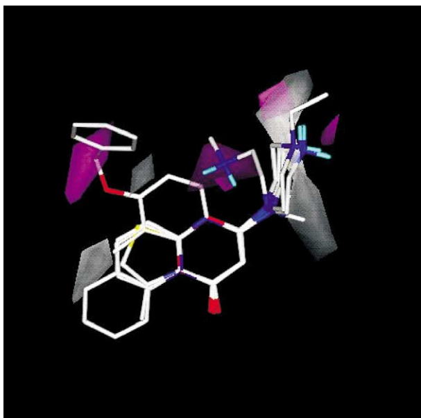
Figure 2. STDEVxCOEFF isocontour electrostatic plots for models P_3 (for the colour code see text). Contour levels as follows: magenta 0.020; white-grey 0.035; compounds 5g , 15f , 9f , 9 and 2b 3 are shown to help interpretation.
